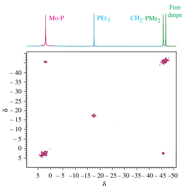
Fig. 7 The ^{31}\text{P}\{-^1\text{H}\}\text{-}^{31}\text{P}\{-^1\text{H}\} COSY NMR spectrum of \text{Mo}_2\text{Cl}_4(\text{dmpe-}P)_4 at 25^\circ\text{C}
